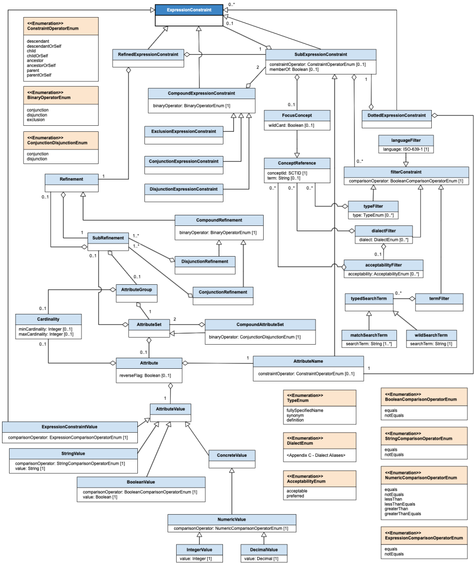
Figure 3: Logical Model of Expression Constraint Language
