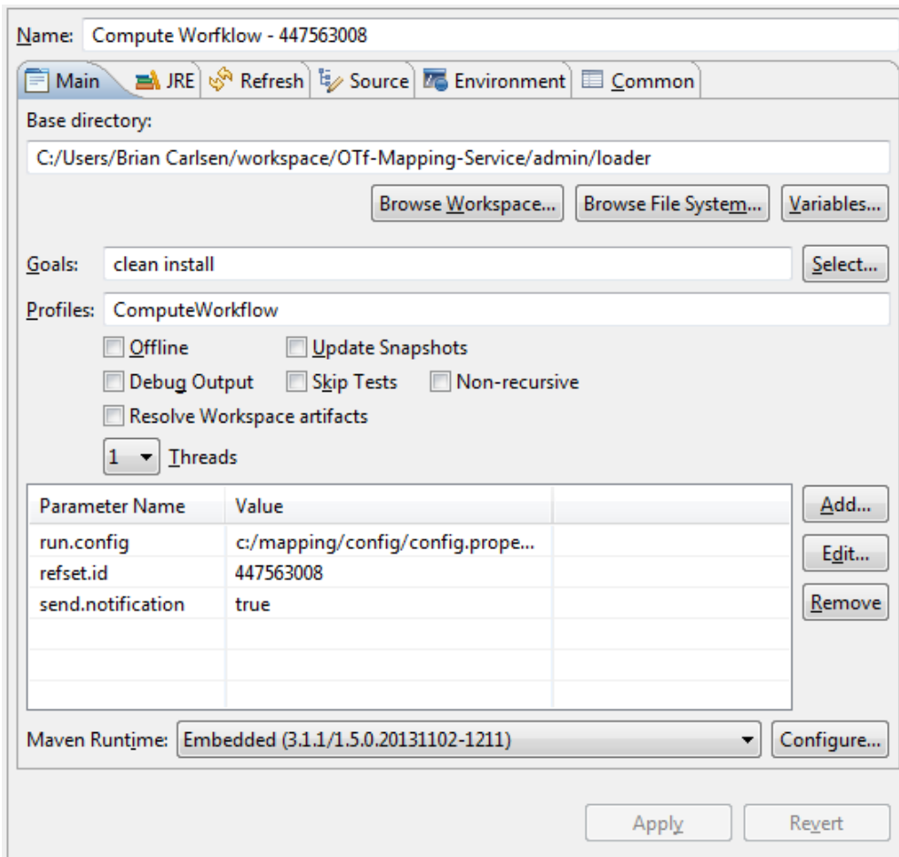
Sample Eclipse run configuration to clear workflow for refset id 447563008:
