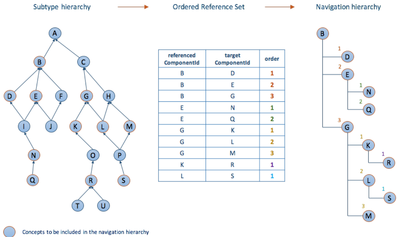
Figure 5.5-1: Ordered reference set example.
