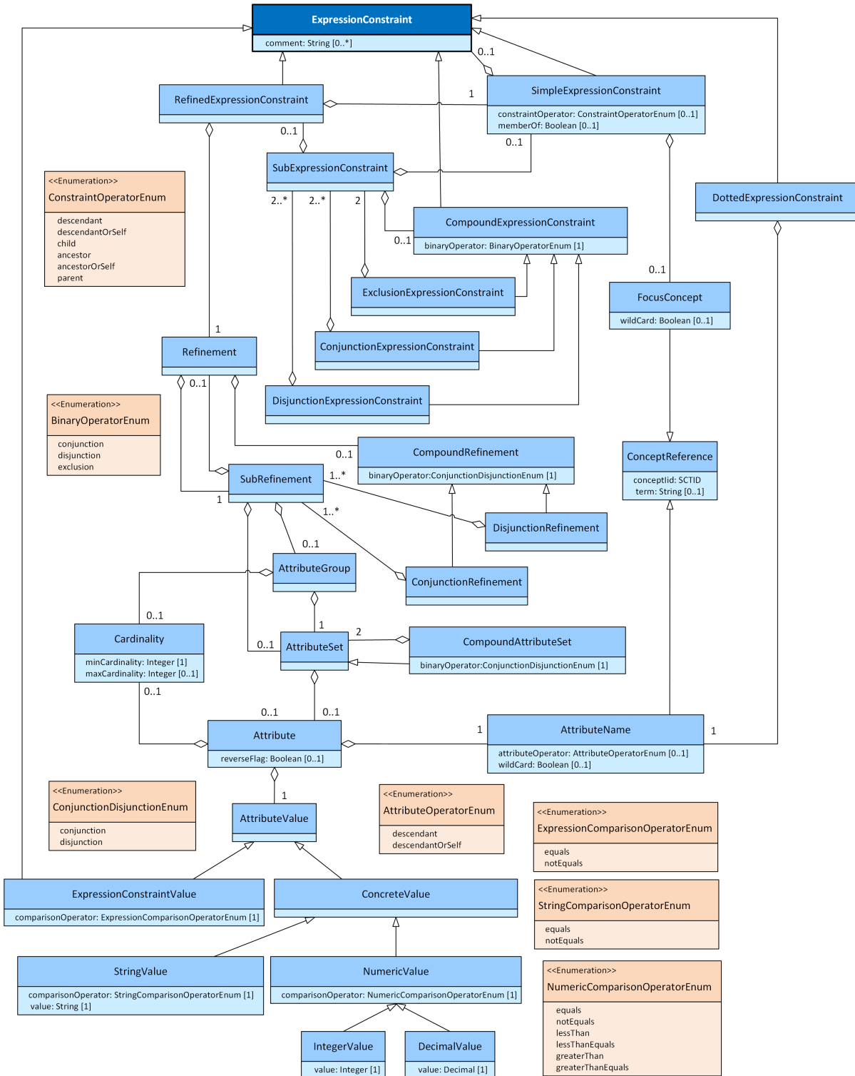
Figure 3: Logical Model of Expression Constraint Language
