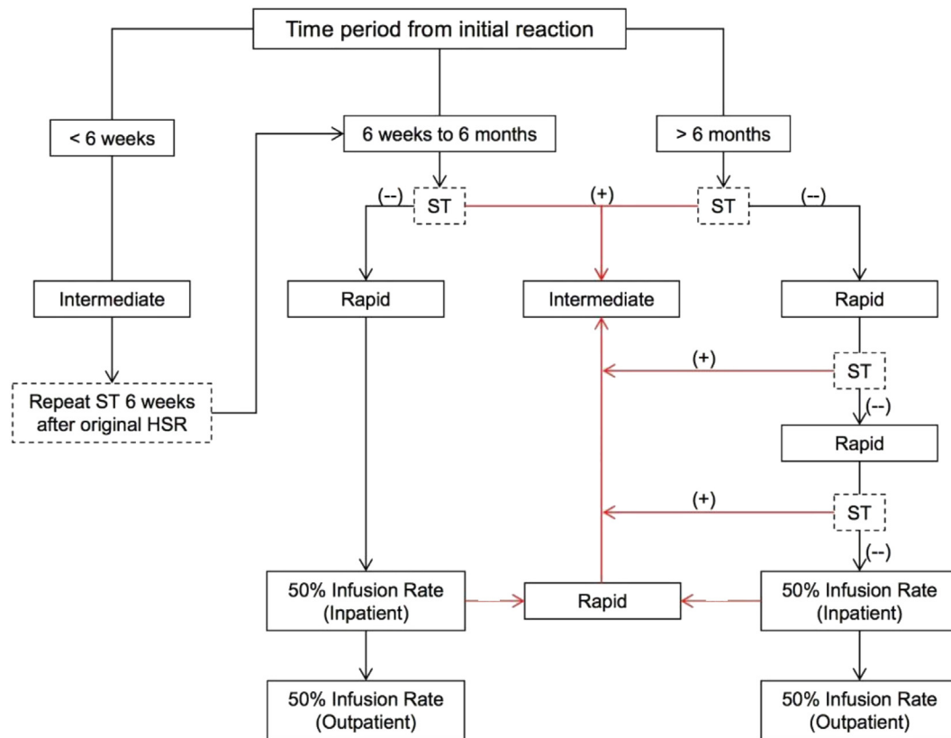
FIG 5. Sample risk stratification after a carboplatin HSR. 501 This risk-stratification algorithm follows an individual patient from the time of the initial HSR through repeat evaluations including skin test (ST) and subsequent treatment steps. ST is performed in between treatments (approximately every 3 weeks). “Intermediate” refers to a standard 12-step desensitization protocol; “rapid” refers to a standard 8-step desensitization protocol; and “50% infusion rate” implies slowing the initial infusion rate by 50%.
