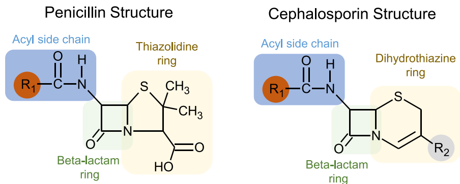
FIG 2. Penicillins and cephalosporins share common structures that are thought to be the source of cross-reactivity: (1) beta-lactam ring, shown in green; (2) side chain, or R group with R1 location shown in red and R2 location shown in gray. Cross-reactivity is largely based on R1 side chains, with identical side chains in patients with IgE-mediated allergy posing the highest risk. Rarely, cross-reactivity has been demonstrated through R2 side chains and the beta-lactam ring (see Table XII).
