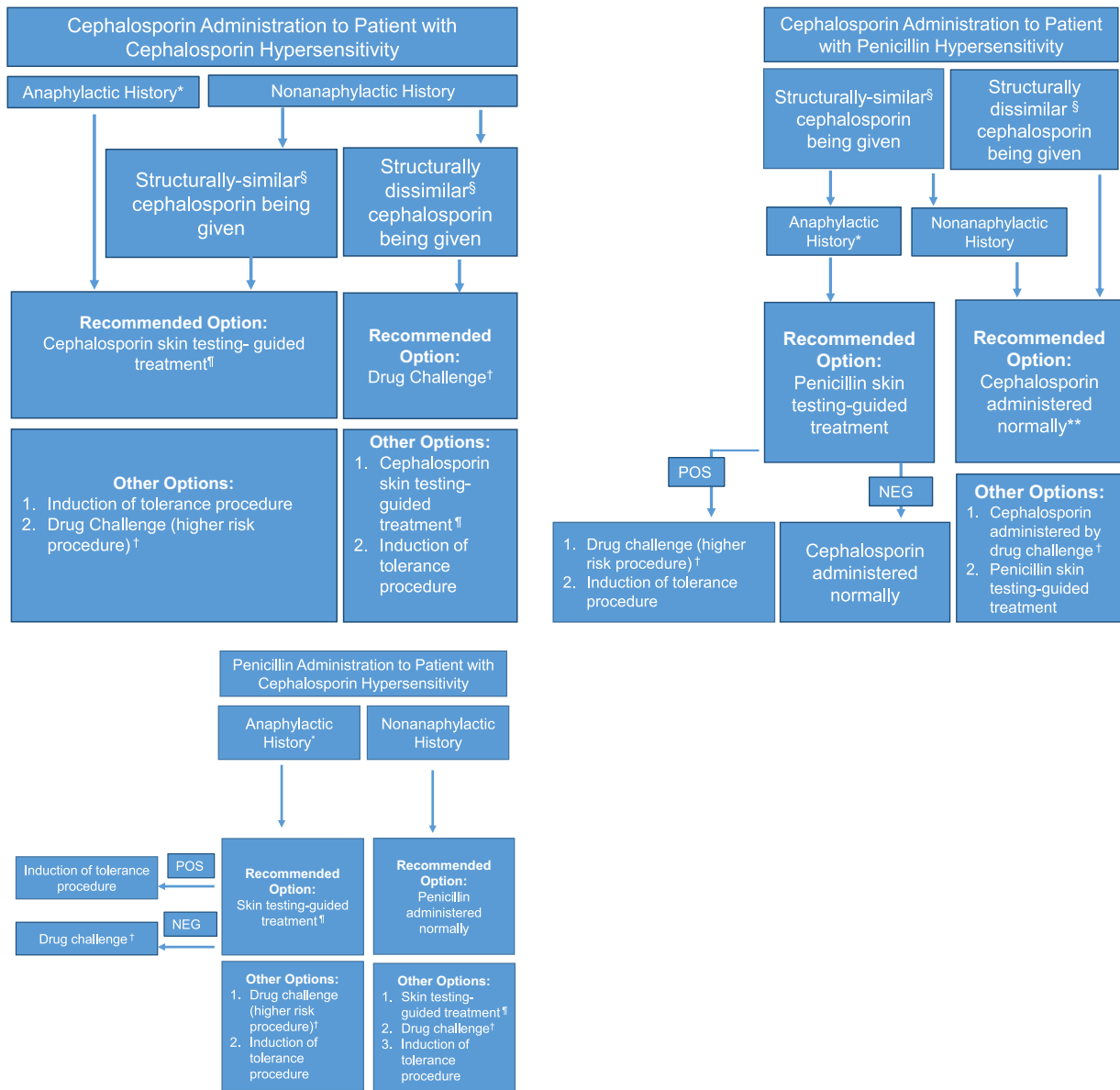
FIG 3. Recommended approach to beta-lactam administration in patients with prior beta-lactam allergies.
